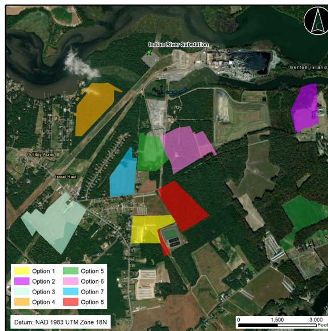
Figure 2-22. Optional US Wind Substation Locations in the Vicinity of Indian River Substation
