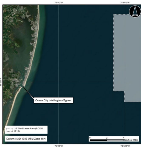
Figure 2-23. Ocean City Inlet Operations Site
