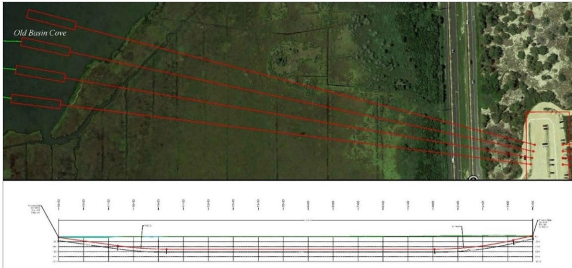
Figure 3-11. HDD Profile Offshore/Onshore Transition Vault to Indian River Bay
