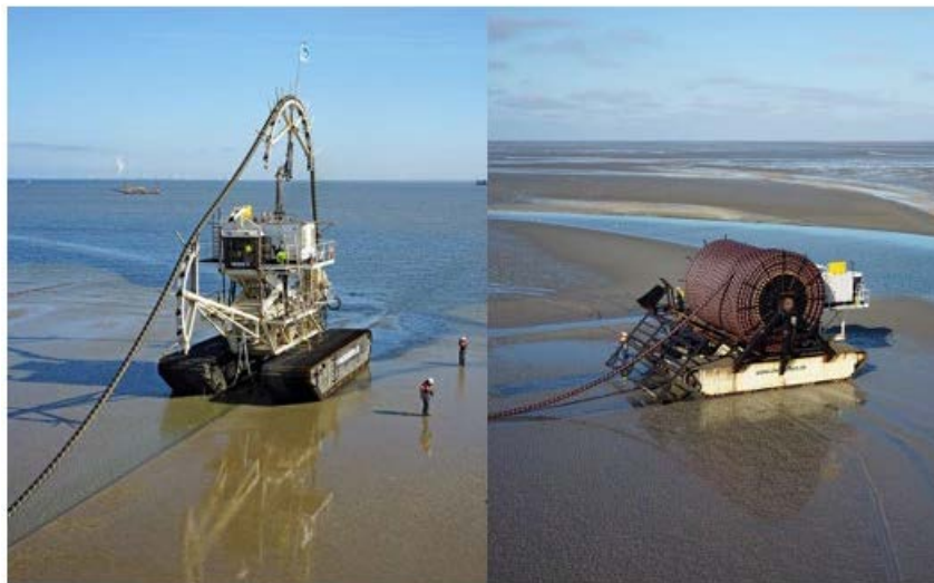
Figure 3-8. Examples of Near Shore Cable Installation ¶Source: www.geminiwindpark.nl
