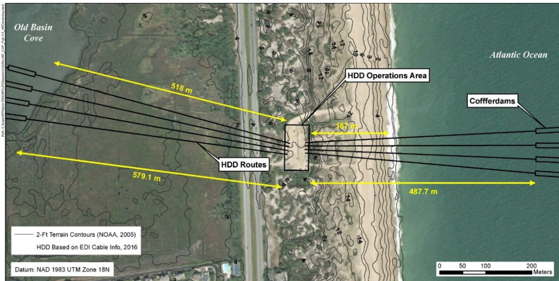
Figure 3-10. Preliminary Onshore Export Cable Corridor 1 Plan: HDD with Offshore/Onshore Transition Vault Connection
